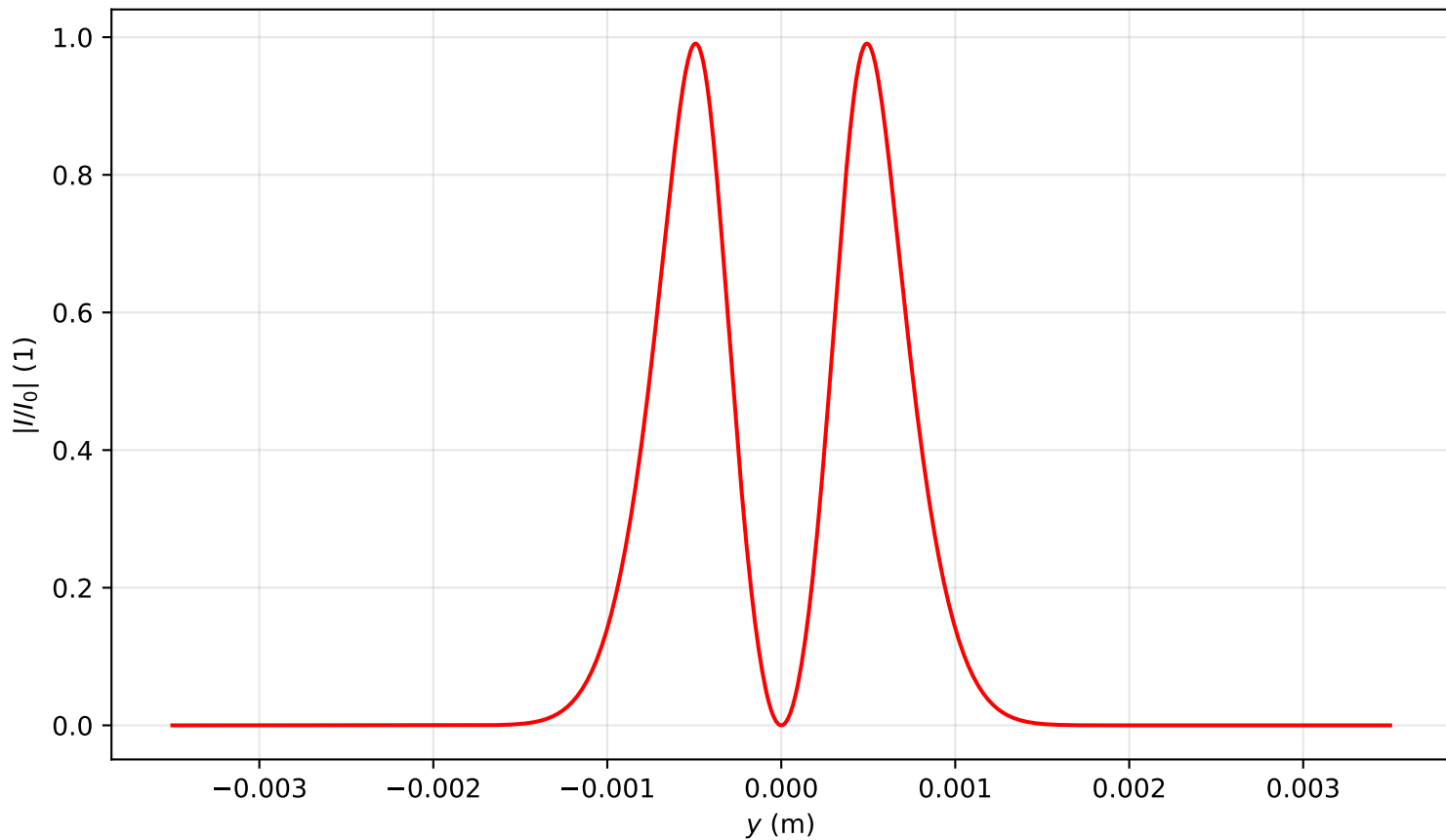
Intensity profile I(x=0, y, z=0.159)/I_0 , \text{Pin}=9.0\text{Pcr} , artificial time
